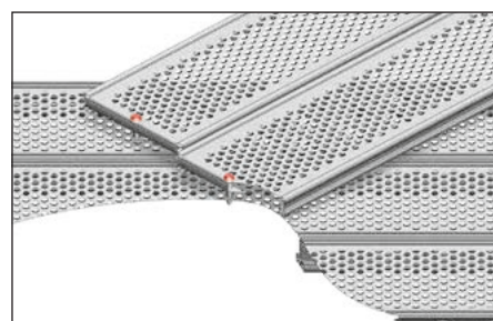
2 locking pins or 1 securing screw for each support secure the steel plank against slipping and lifting off.
