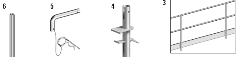
Assembly with guardrail post , scaffolding tubes and double couplers
