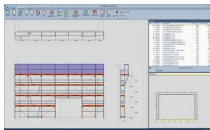
Speedy facade scaffolding with console brackets, brick guards and drive-trough cut-out
