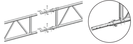
Coupler connection as in sketch possible for Ref. No. 4902
